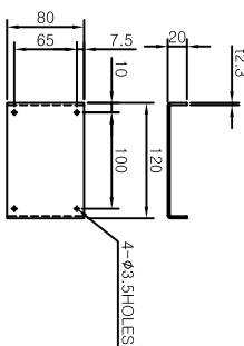
DETAIL OF BRACKET NAME PLATE
