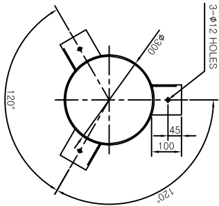
DETAIL OF LEG
