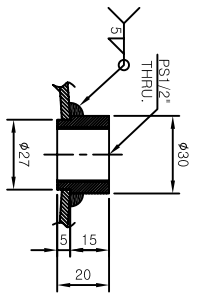
DETAIL OF SOCKET[15A]
