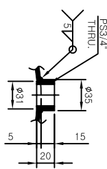
DETAIL OF SOCKET[20A]
