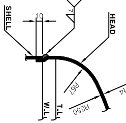
DETAIL OF "B"
