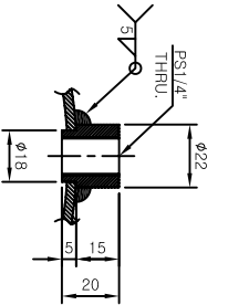
DETAIL OF SOCKET[8A]
