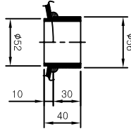
DETAIL OF SOCKET[40A]
