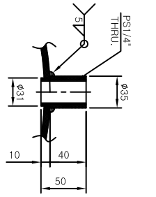
DETAIL OF SOCKET [20A] [SCALE=1:4]
