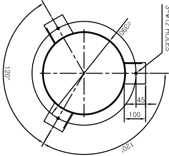
DETAIL OF LEG
