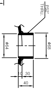
DETAIL OF SOCKET [50A] [SCALE=1:4]
