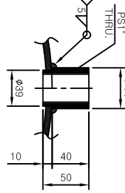
DETAIL OF SOCKET [25A] [SCALE=1:4]
