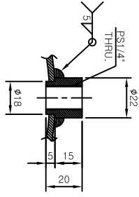
DETAIL OF SOCKET [18A] [SCALE=1:2]
