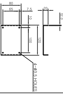
DETAIL OF BRACKET NAME PLATE [SCALE=1:8]
