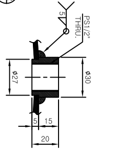
DETAIL OF SOCKET [15A] [SCALE=1:2]
